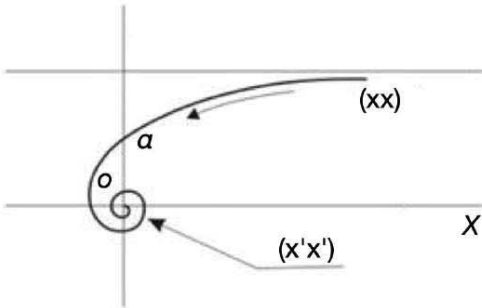
Hyperbolic spiral \rho \theta = a
